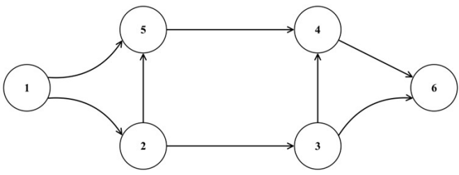
Fig 1: Directed acyclic graph (DAG) diagram containing 6 nodes, labelled from one to six. Directed edges connect the nodes.
