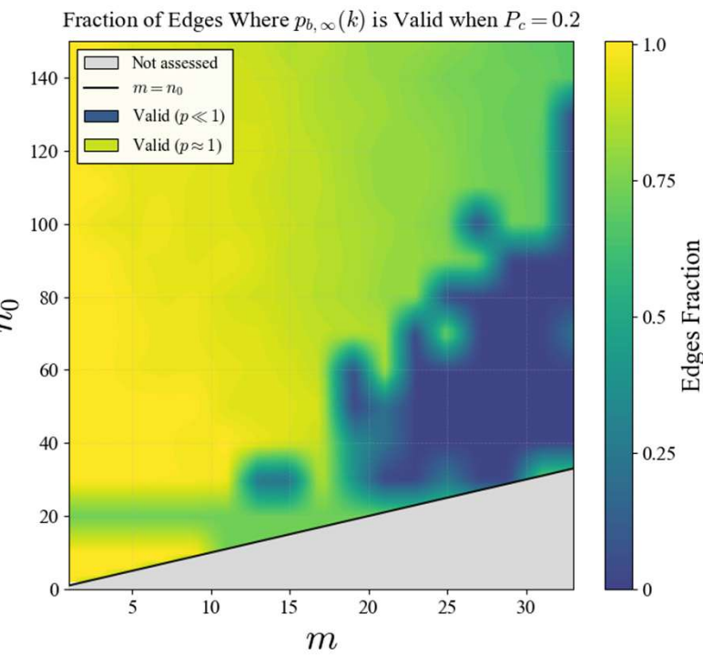
Figure 5. Fraction of total citations for which equation (1) passes our G.o.F test as a function of m citations each paper makes, (horizontal axis) and the n_0 initial nodes in our model, (vertical axis). The colour scale shows the fraction of edges retained, from 0 (dark) to 1 (bright yellow), where a value of 1 indicates that all edges are within the regime where our G.o.F test accepts the theoretical distribution at the chosen threshold P_c . 10,000 nodes added.
