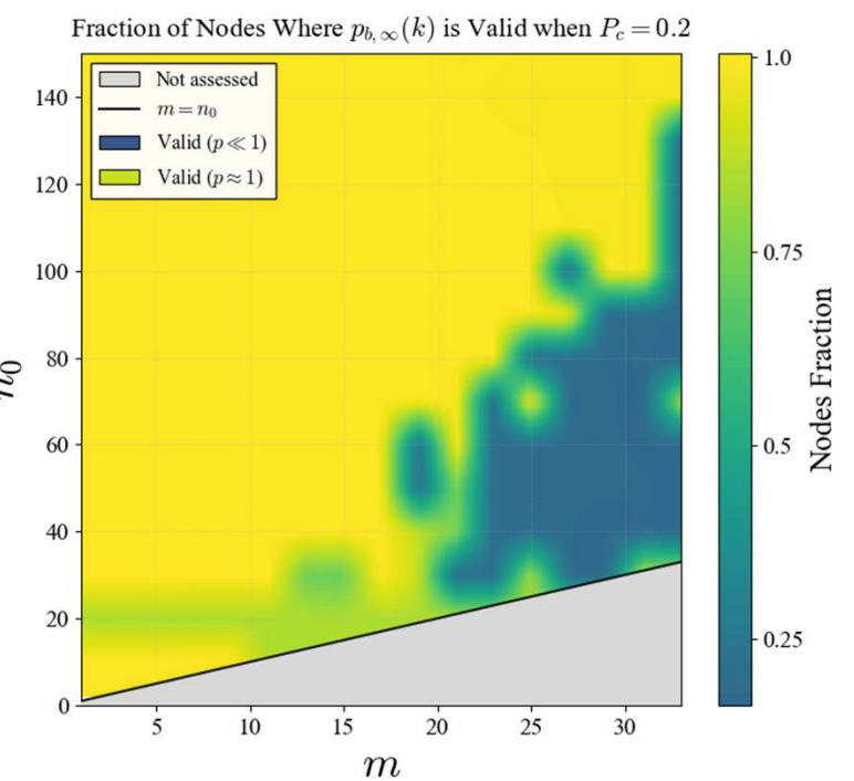
Figure 6. Fraction of papers for which equation (1) passes our G.o.F test as a function of m citations each paper makes, (horizontal axis) and the n_0 initial papers in our model, (vertical axis). The colour scale shows the fraction of papers retained, from 0 (dark) to 1 (bright yellow), where a value of 1 indicates that all papers are within the regime where our G.o.F test accepts the theoretical distribution at the chosen threshold P_c . 10,000 nodes added.
