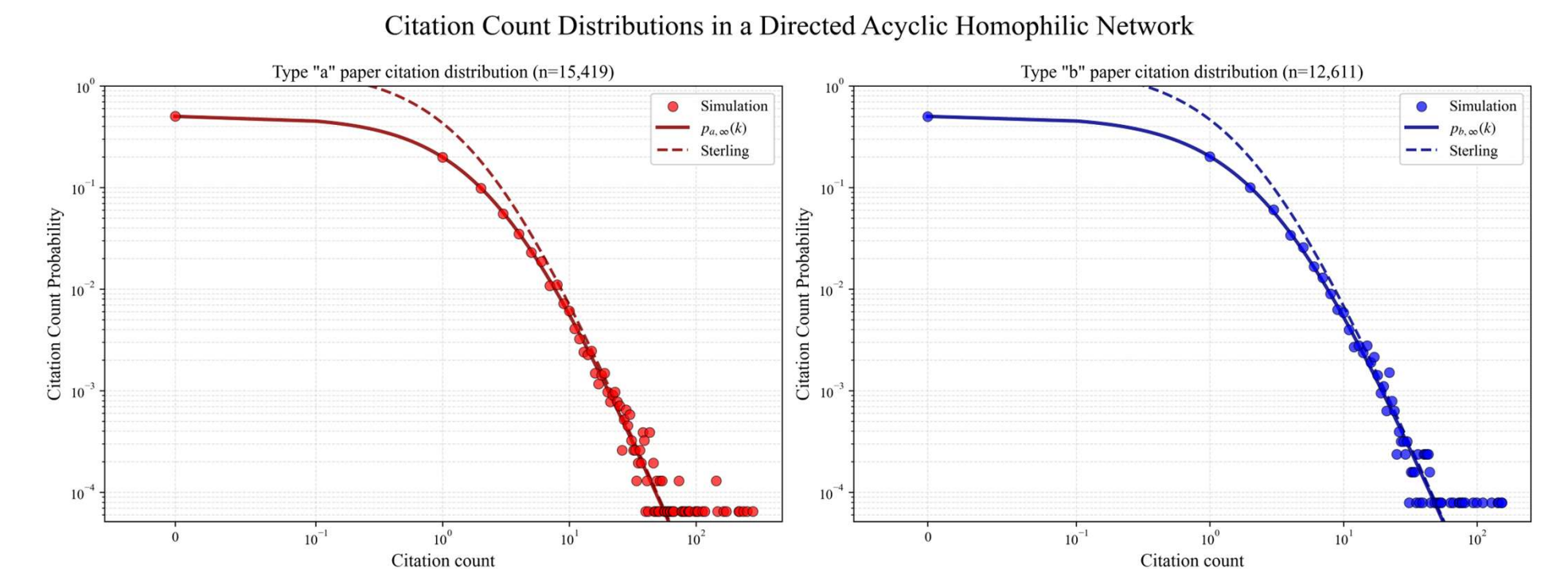
Figure 4. Log-binned citation count distributions for node types “a” and “b” in a directed acyclic homophilic network. Empirical probabilities are computed using logarithmic binning with binning factor 1.01; bin centres are given by the geometric mean. The k = 0 mass is shown separately. The x-axis is displayed on a symmetric logarithmic scale (linear for |k| < 0.1 , logarithmic otherwise), while the y-axis is logarithmic. Overlaid curves show the corresponding theoretical distributions. Network parameters: N = n_0 + 28,000 , n_0 = 3 , m = 2 , h = 0.7 , and type fraction f_a = 0.55 .
